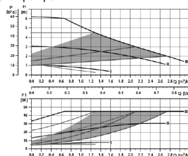
Alpha2 pumpe
